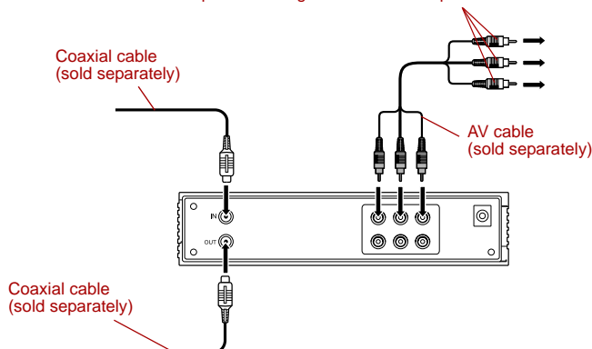
Connection method for the computer and set-top box
