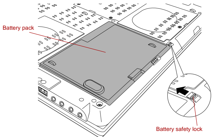
Releasing the battery pack (1)
