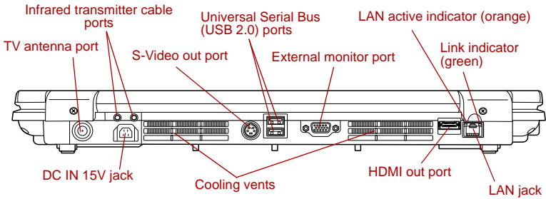
The back of the computer
