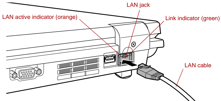
Connecting the LAN cable
