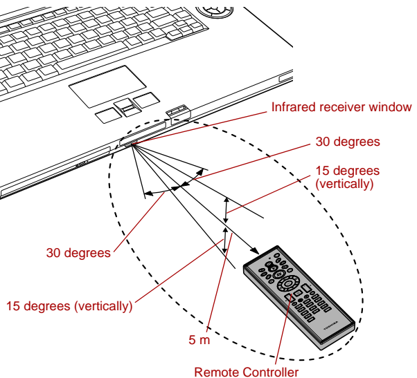
Operational range of the remote control
