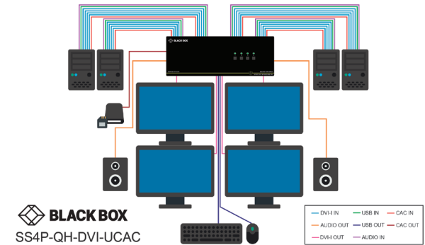
FIGURE 2. QUAD-HEAD APPLICATION DIAGRAM
