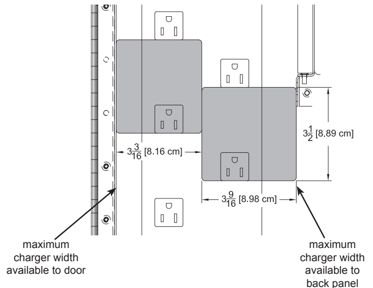
nominal outlet spacing on each 16-outlet power unit
