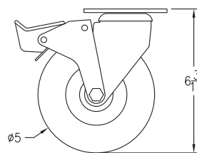
5" balloon wheel (BW)
