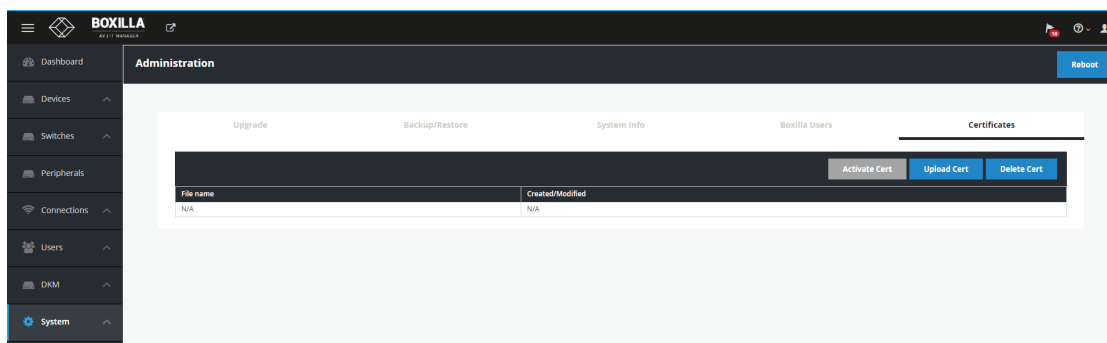
FIGURE 13-12. DELETE SUCCESSFUL
