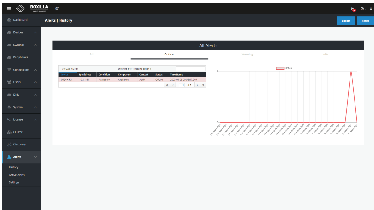
FIGURE 16-2. CRITICAL
