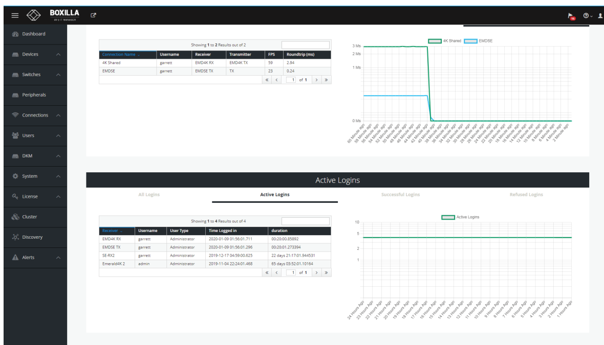
FIGURE 17-2. ACTIVE LOGINS
