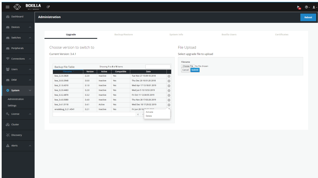
FIGURE 13-7. SYSTEM SCREEN—UPGRADE
