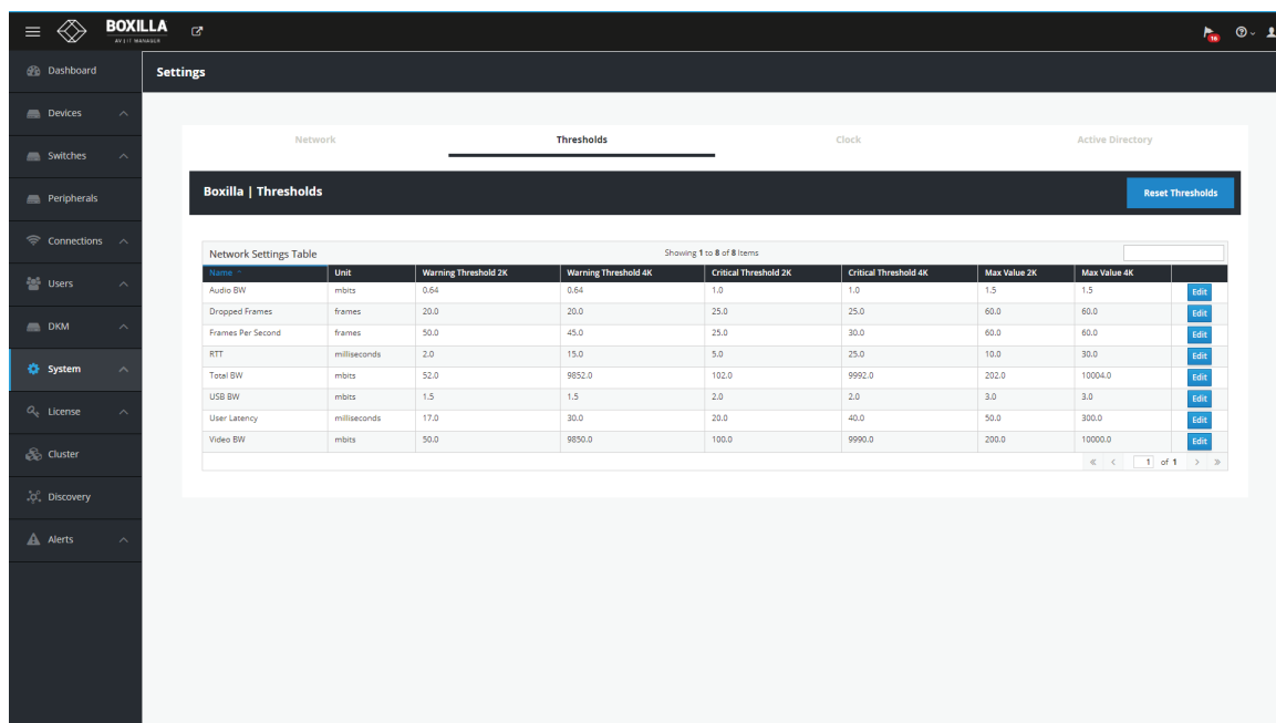
FIGURE 13-14. ALERT THRESHOLDS
