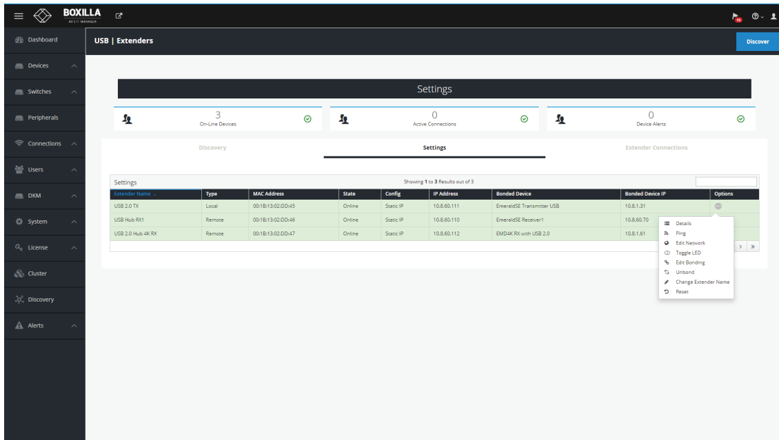
FIGURE 9-10. OPTIONS MENU
