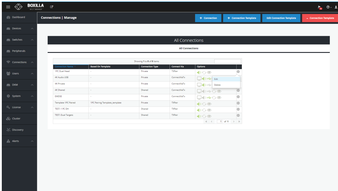
FIGURE 10-7. CONNECTIONS
