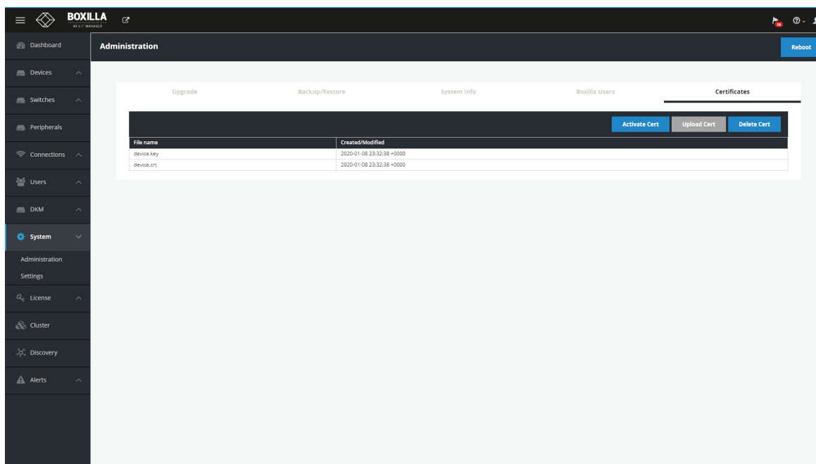
FIGURE 13-8. CERTIFICATES TAB
