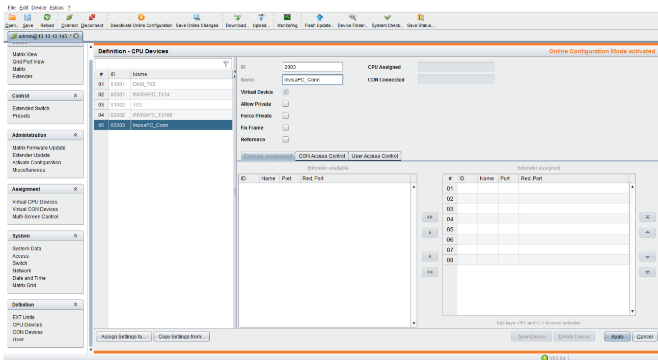
FIGURE 12-3. NAME VIRTUAL CPU SCREEN
