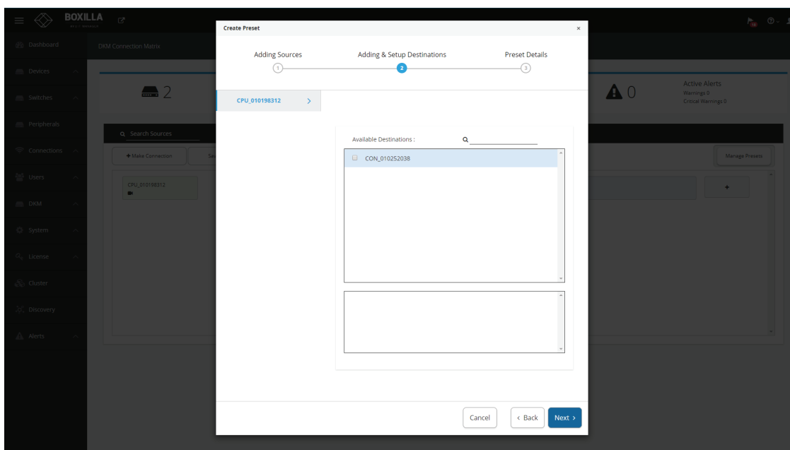
FIGURE 12-24. SELECT DESTINATIONS
