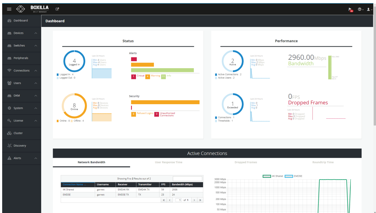
FIGURE 17-1. DASHBOARD TOP
