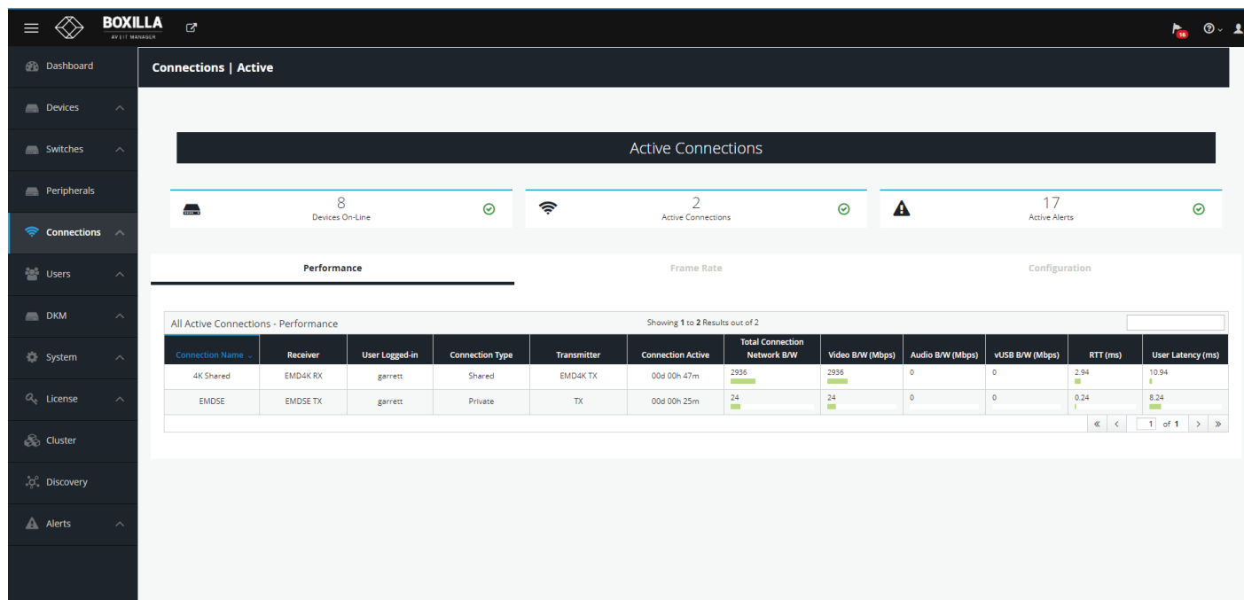
FIGURE 10-19. ACTIVE CONNECTIONS
