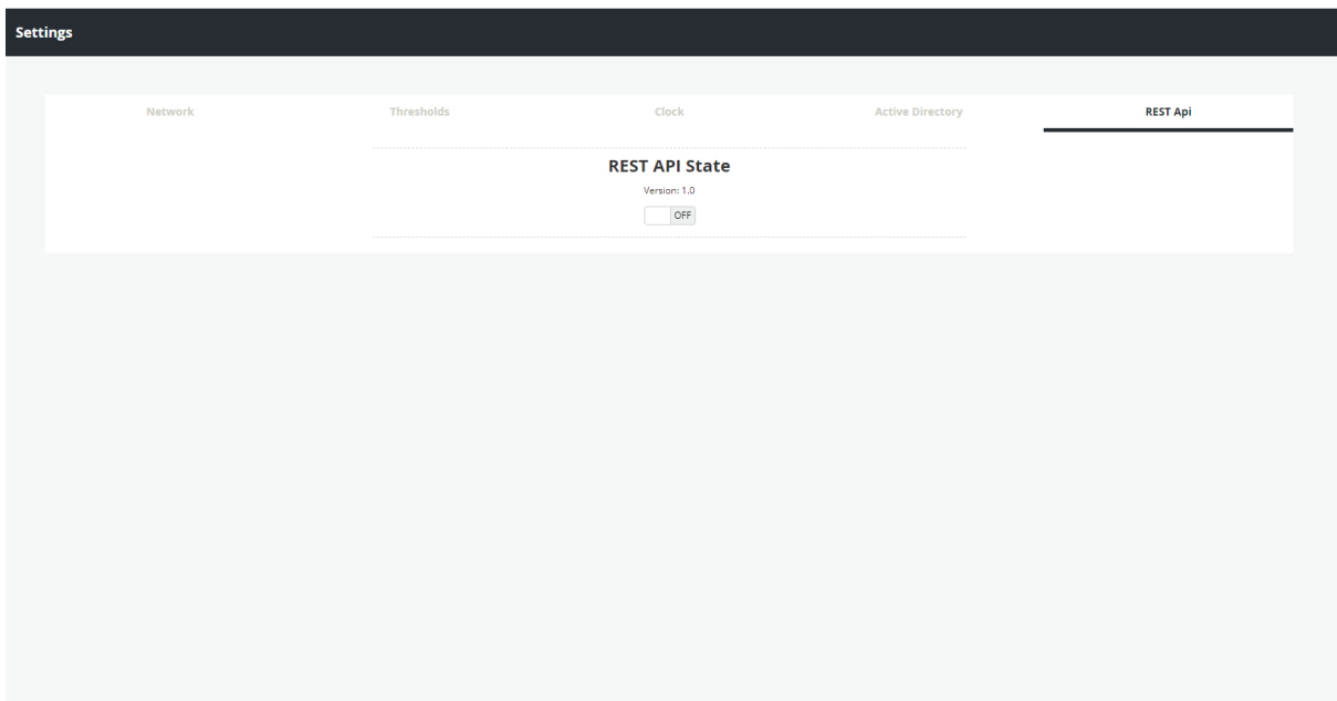
FIGURE 13-23. API OFF
