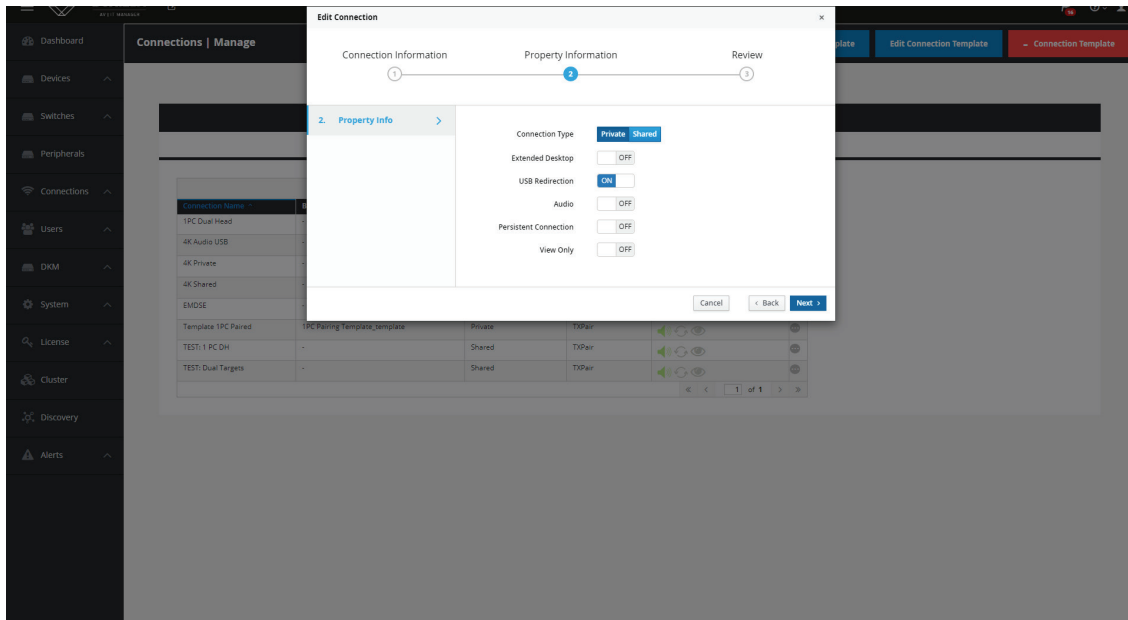
FIGURE 10-8. EDIT CONNECTION
