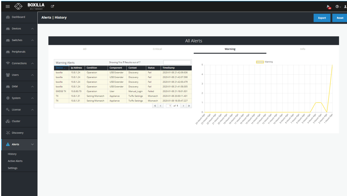
FIGURE 16-3. WARNING
