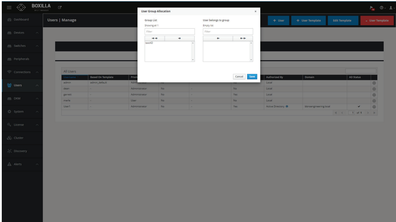
FIGURE 11-10. MANAGE GROUPS
