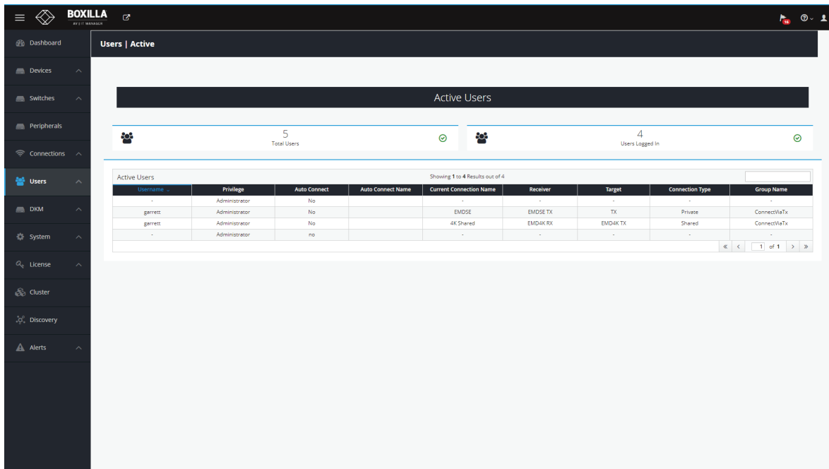
FIGURE 11-9. ACTIVE USERS
