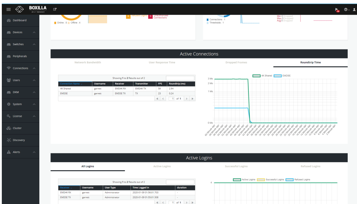
FIGURE 17-4. ROUNDTRIP TIME
