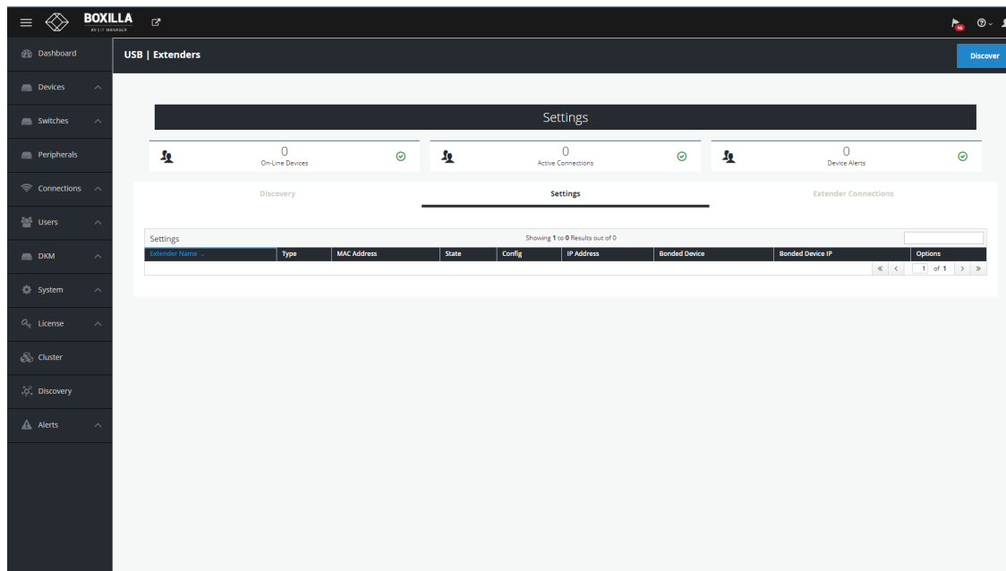
FIGURE 9-8. PERIPHERALS>>SETTINGS TAB
