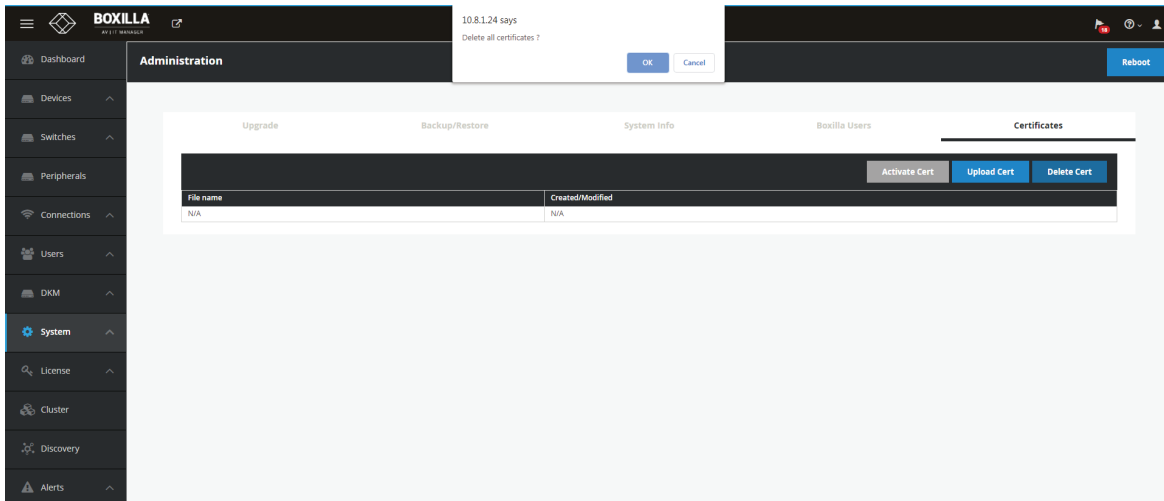
FIGURE 13-11. DELETE BUTTON
