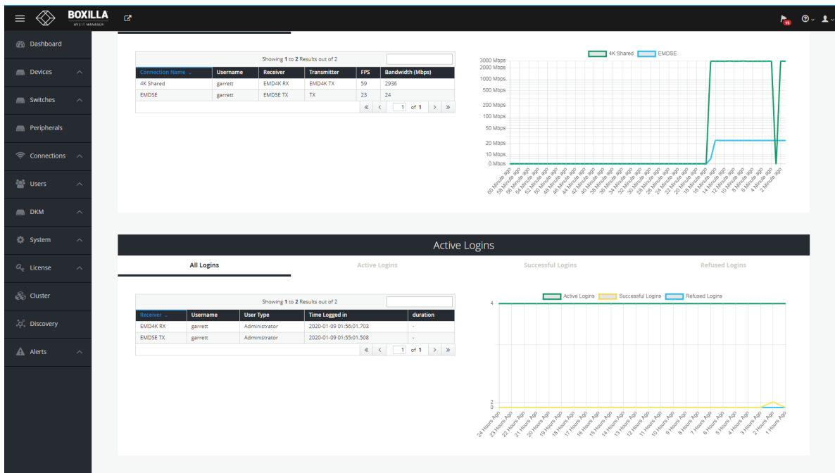
FIGURE 17-5. DASHBOARD BOTTOM
