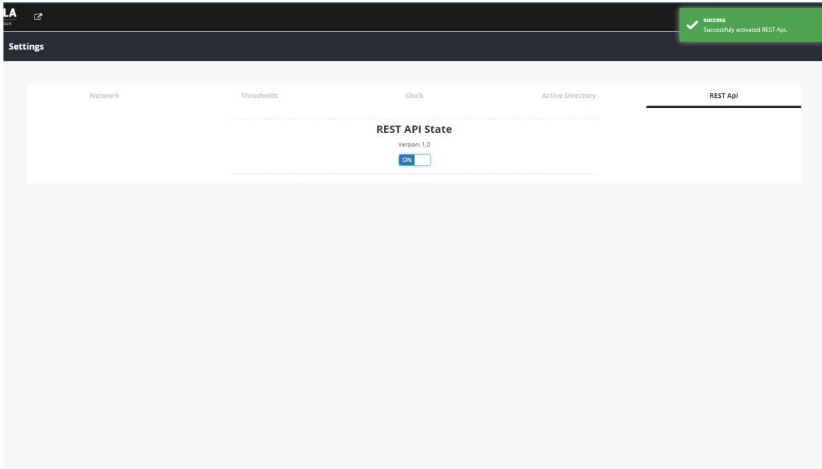
FIGURE 13-22. API ON
