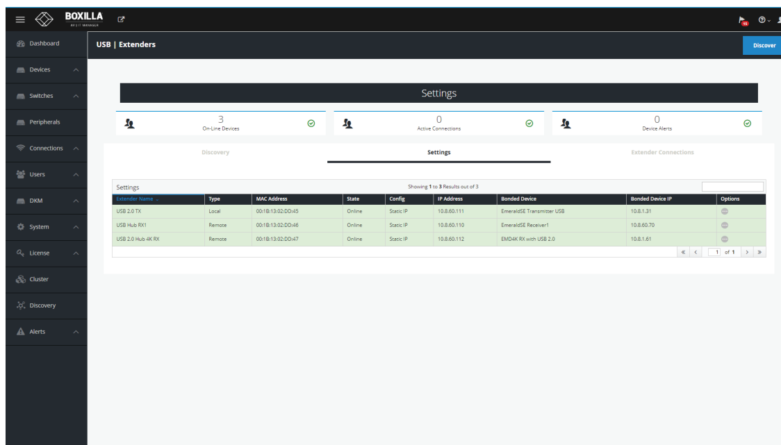
FIGURE 9-9. DEVICE DETAILS
