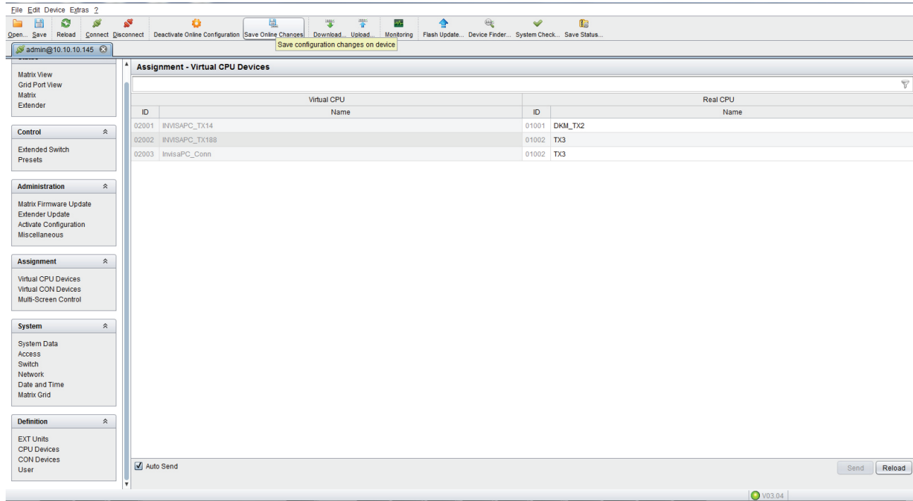
FIGURE 12-5. SAVED CHANGES
