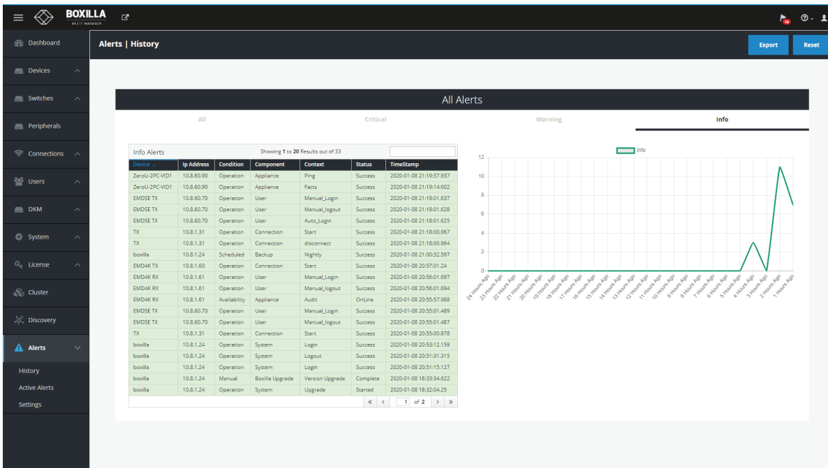
FIGURE 16-4. INFO
