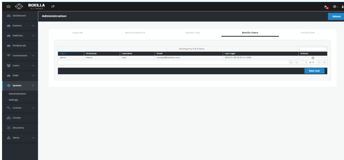
FIGURE 13-18. SYSTEM USERS
