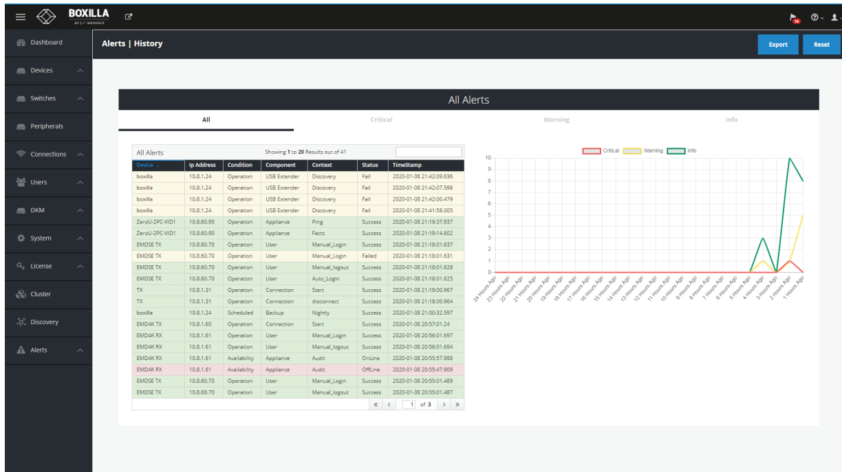
FIGURE 16-1. ALERTS HISTORY
