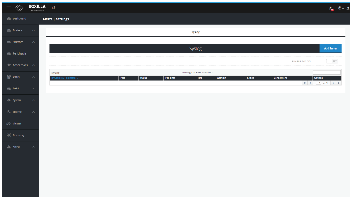
FIGURE 16-5. SYSLOG
