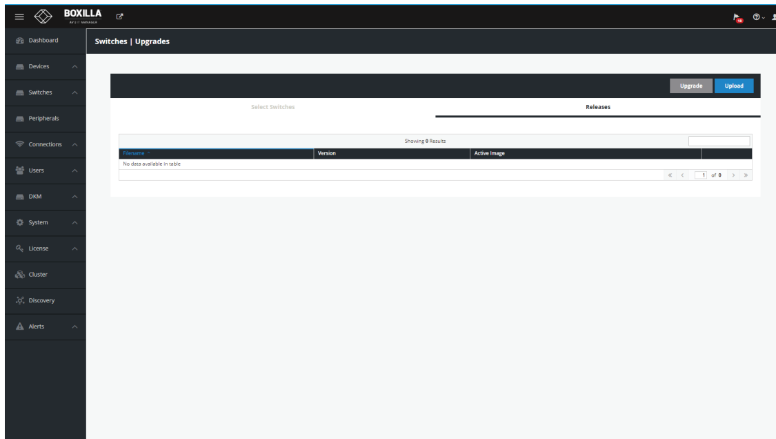
FIGURE 8-23. ACTIVATE RELEASE
