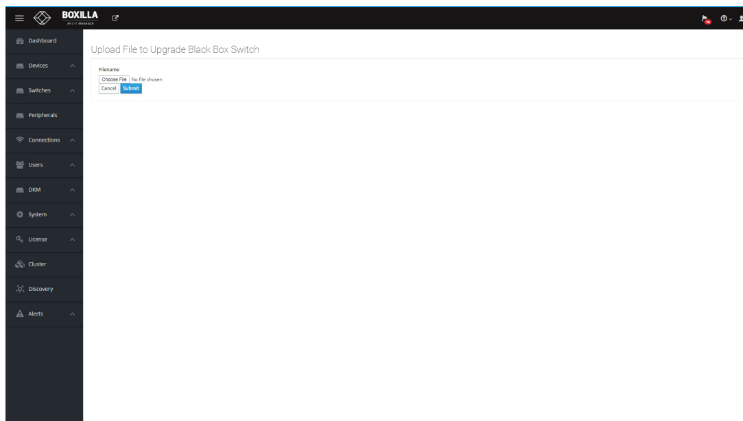
FIGURE 8-24. UPLOAD RELEASE
