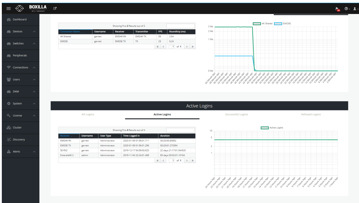
FIGURE 17-6. ACTIVE LOGINS
