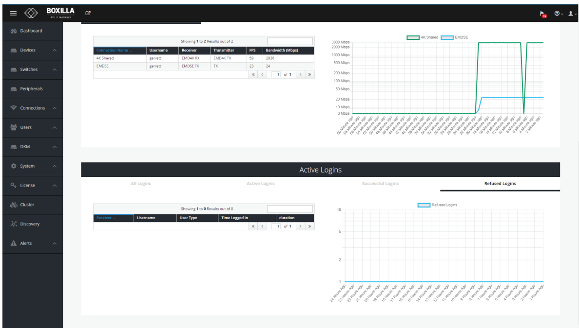
FIGURE 17-8. REFUSED LOGINS
