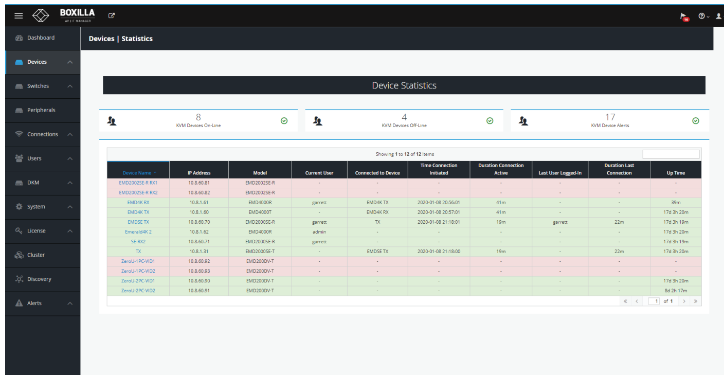
FIGURE 7-15. DEVICE STATISTICS
