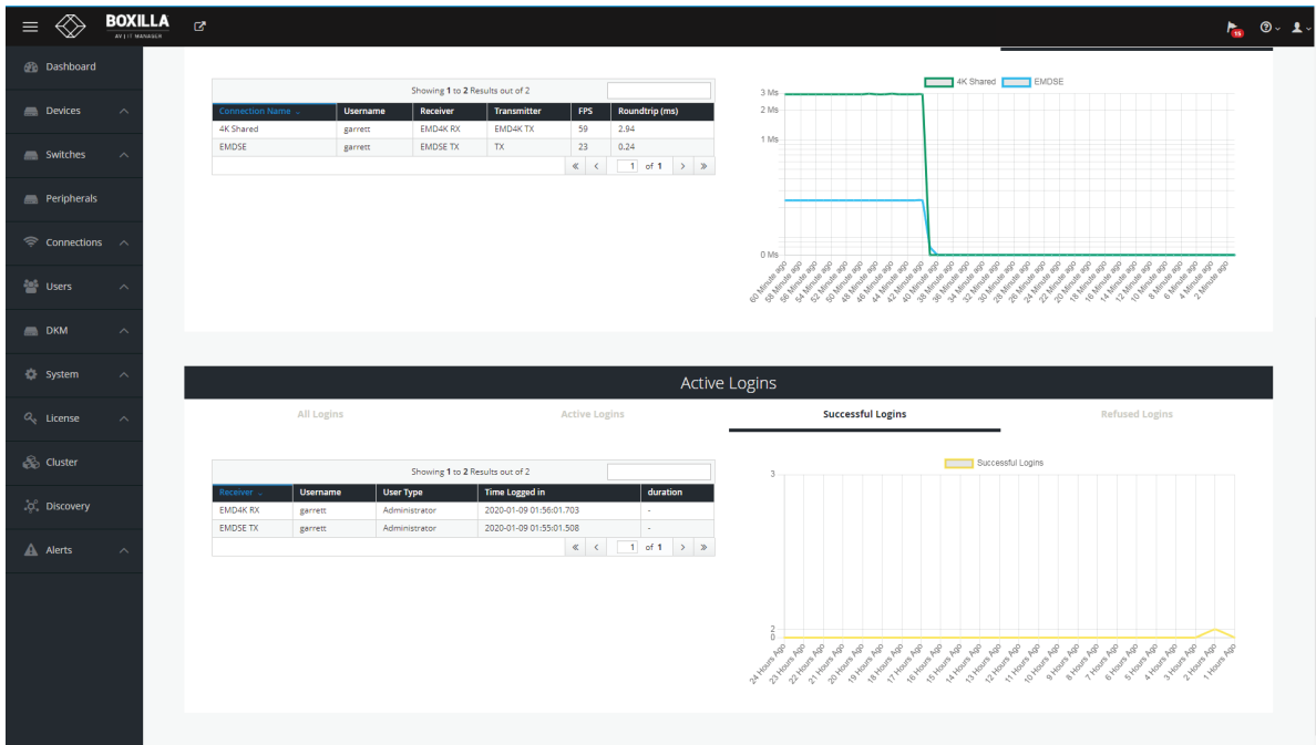
FIGURE 17-7. SUCCESSFUL LOGINS
