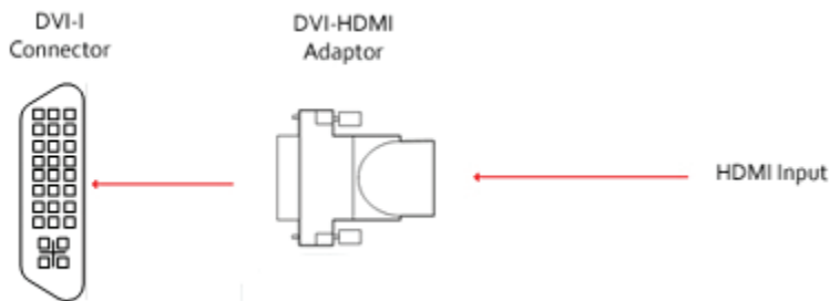
Figure B-29. HDMI input.
