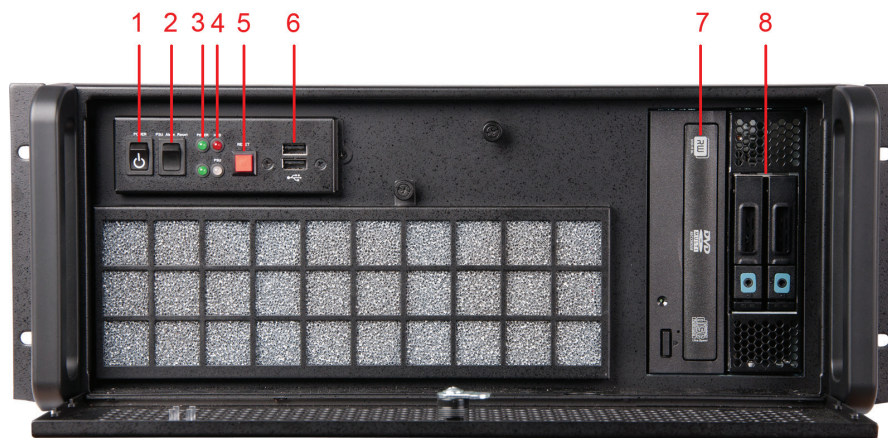
Figure 2-5. Front panel of the VWP-2090.
