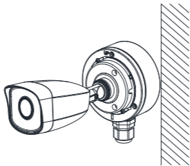
Figure 2-7 Combine Junction Box's Cover with its Body
