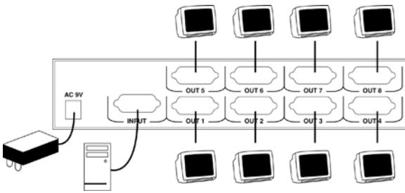
Figure 3: ST128PRO Connection
