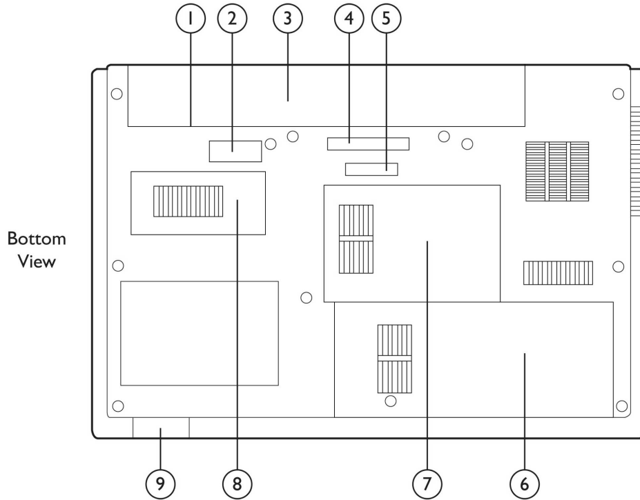
Bottom View
