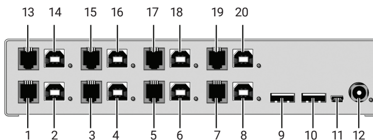
FIGURE 2-3. REAR VIEW OF THE ACX1008A-HID2
