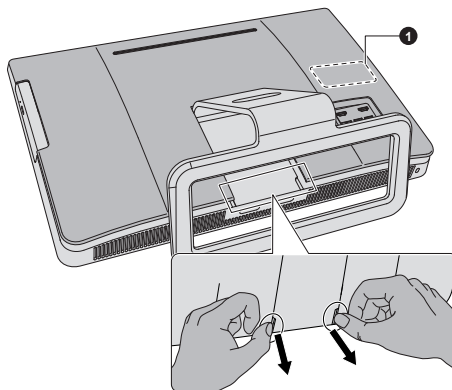
Figure 4-14 Removing the back cover
