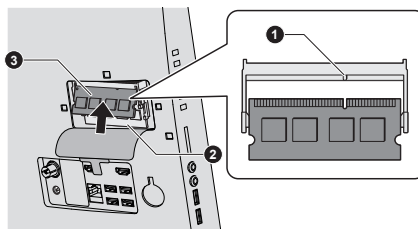
Figure 4-15 Seating the memory module
