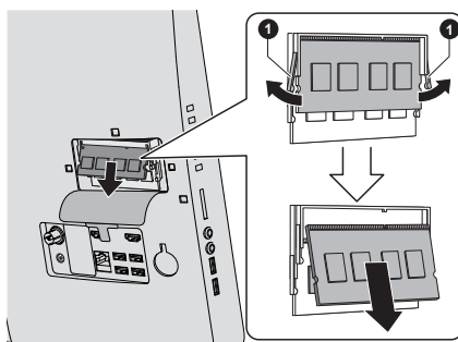
Figure 4-16 Removing the memory module
