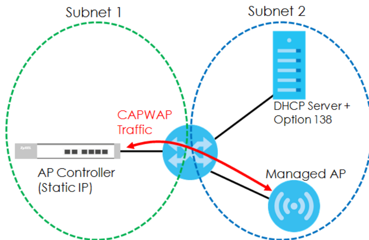
Figure 36 CAPWAP and DHCP Option 138
