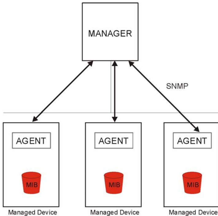
Figure 103 SNMP Management Model
