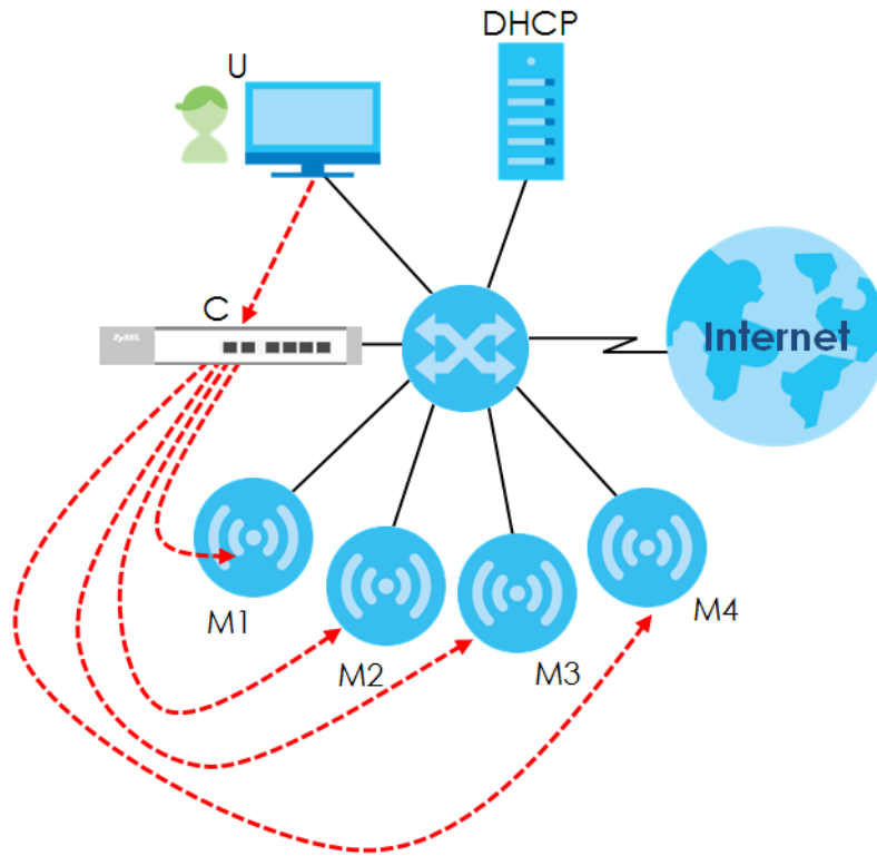
Figure 35 CAPWAP Network Example
