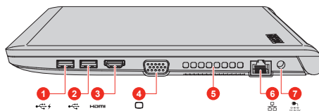
Figure 3-9 The right side of the computer (A40-C/R40-C)
