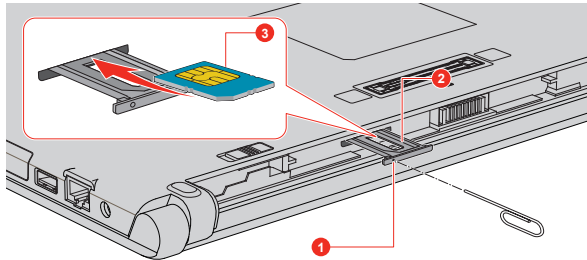
Figure 4-8 Open the SIM card tray with the eject hole (A30-C)
