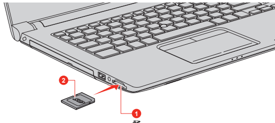
Figure 4-19 Inserting memory media (A40-C/R40-C)
