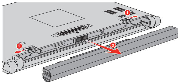
Figure 4-7 Releasing the battery pack (A30-C)
