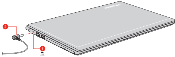
Figure 2-4 Connecting the DC output plug to the computer (A40-C/R40-C)
