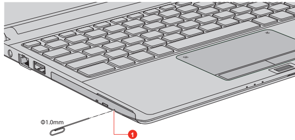
Figure 4-6 Manual release with the eject hole (A30-C)
