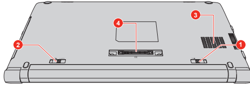
Figure 3-11 The underside of the computer (A40-C/R40-C)
