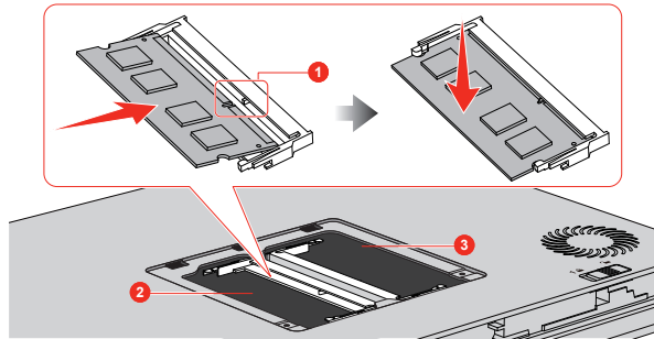
Figure 4-12 Seating the memory module
