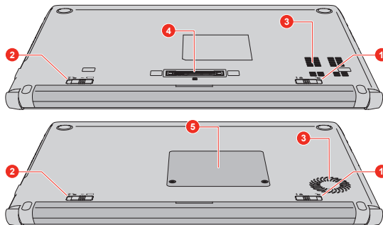
Figure 3-5 The underside of the computer (A30-C)
