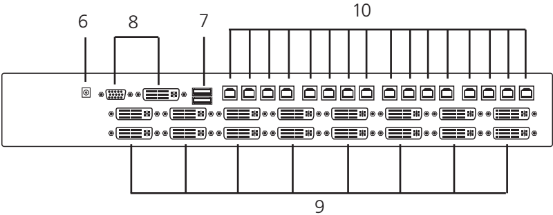
Figure 2-2. KV9516A back panel.
