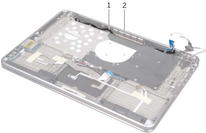
1 camera-cable routing 2 air vent
