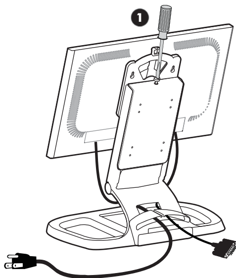
Figure 3-13 Removing the Thumbscrew
