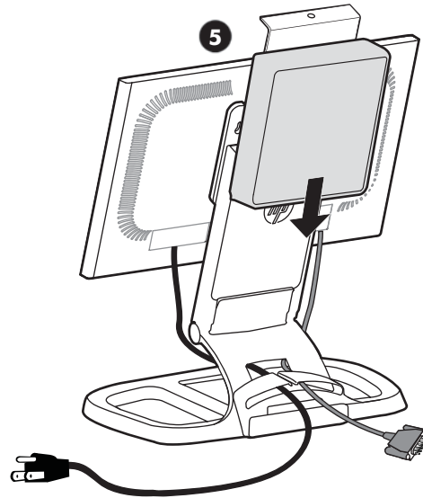
Figure 3-17 Installing a Thin Client
