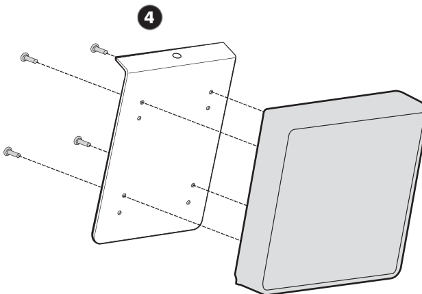
Figure 3-16 Installing the Computer Mounting Bracket
