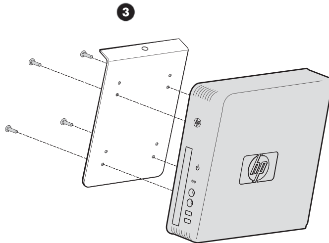
Figure 3-6 Installing the Computer Mounting Bracket
