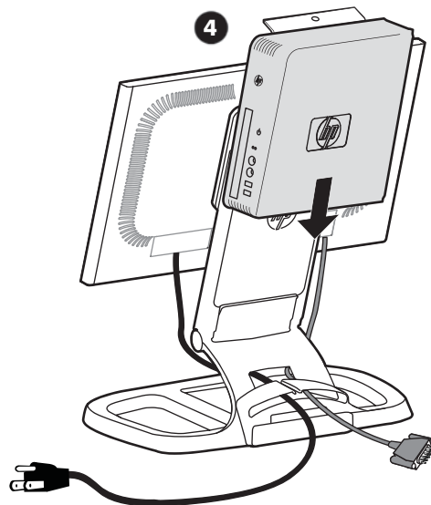
Figure 3-7 Installing a USDT on the Stand
