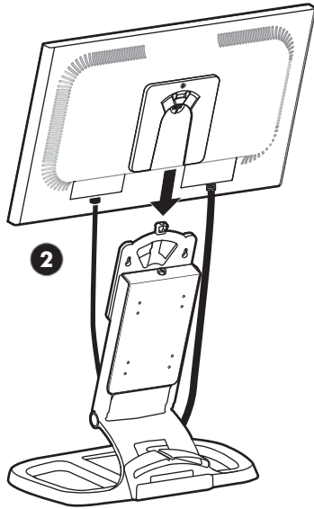
Figure 3-2 Attaching the Monitor
