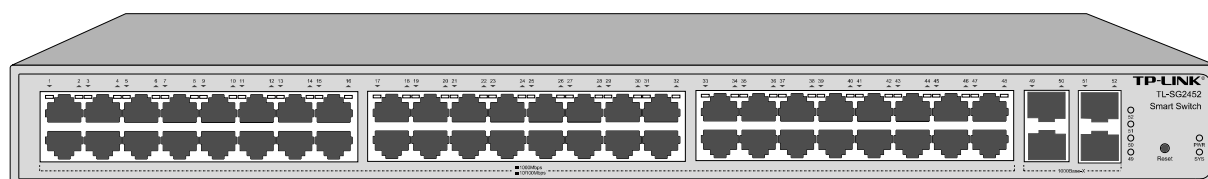
Figure 2-1 Front Panel of TL-SG2452
