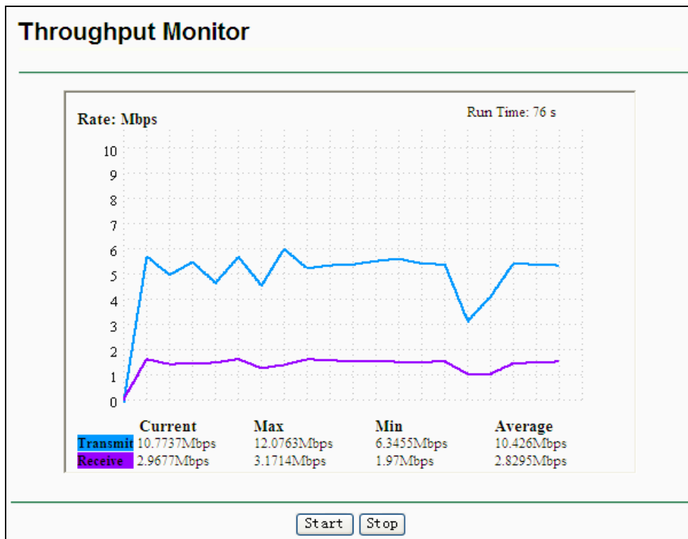
Figure 4-15 Throughput Monitor
