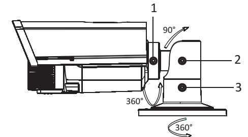
Figure 2-9 3-axis Adjustment
