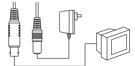
Figure 2-11 The Power Cable & the Video Cable
