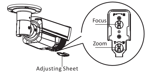
Figure 2-10 Focus and Zoom Adjustment
