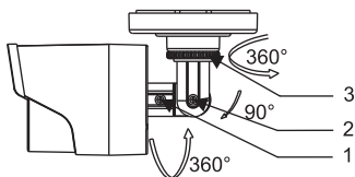
Figure 2-3 3-axis Adjustment
