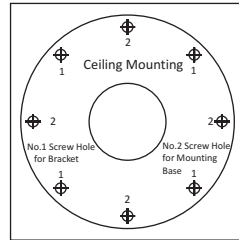
Figure 2-4 Drill Template
