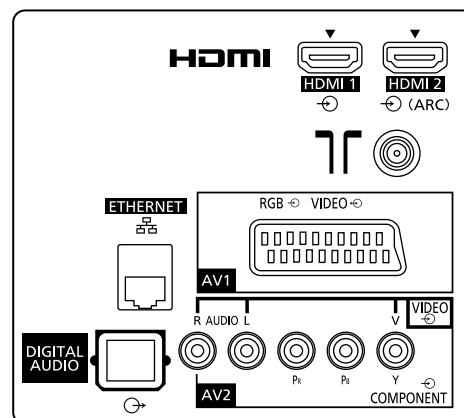
Rear Panel
