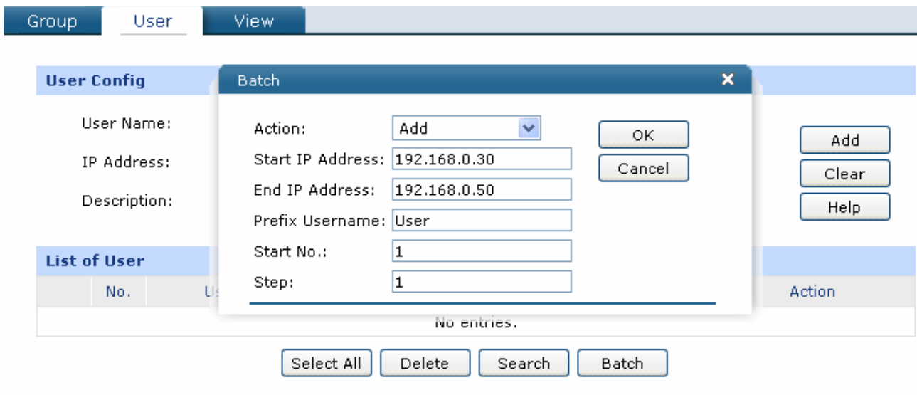
Figure 4-6 User Config - Batch
