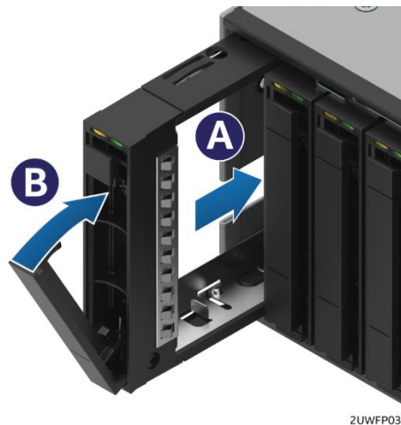
Figure 19. Drive carrier insertion into chassis
