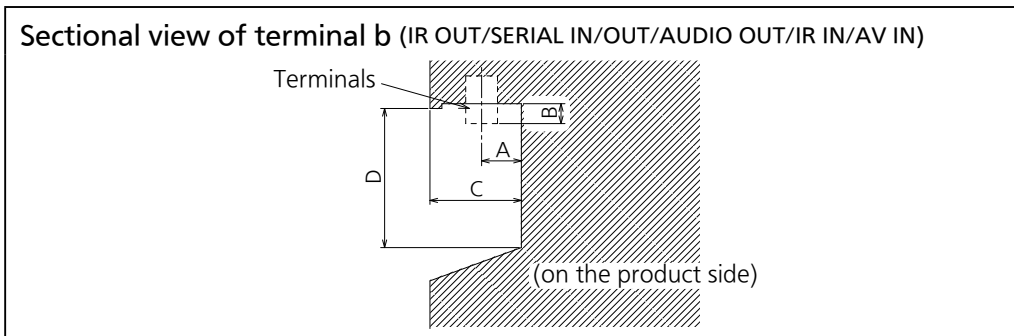
Terminal b 49SF2U Terminal (Bottom)
