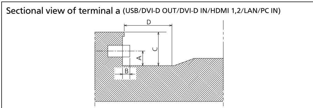
Terminal a 49SF2U Terminal (Side)
