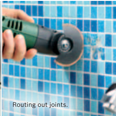
Routing out joints in the tightest of corners.
