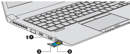
Figure 4-7 Installing the SIM Card (Z40-A)
