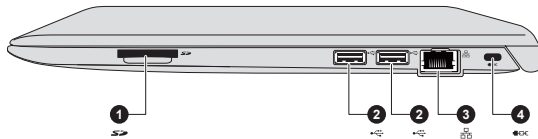
Figure 3-3 The right side of the computer (Z30-A)
