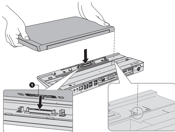
Figure 4-13 Aligning your computer with the Port Replicator (Z30-A)
