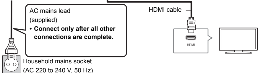
This unit's rear panel
