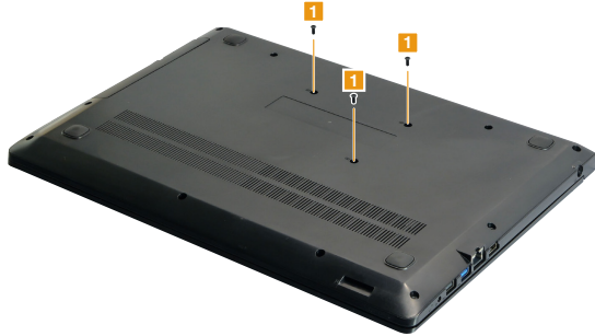
Figure 1. Removal steps of keyboard
