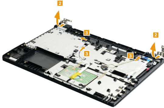
Figure 11. Removal steps of upper case (continued)
