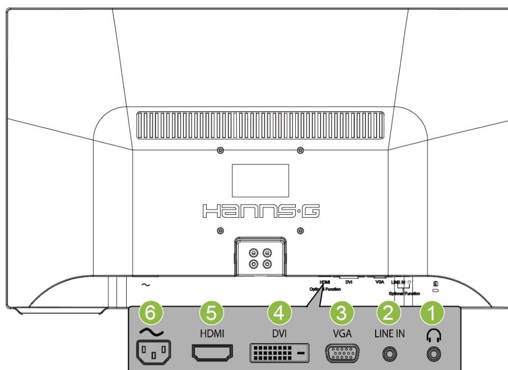
Figure.2. Connecting to a PC
