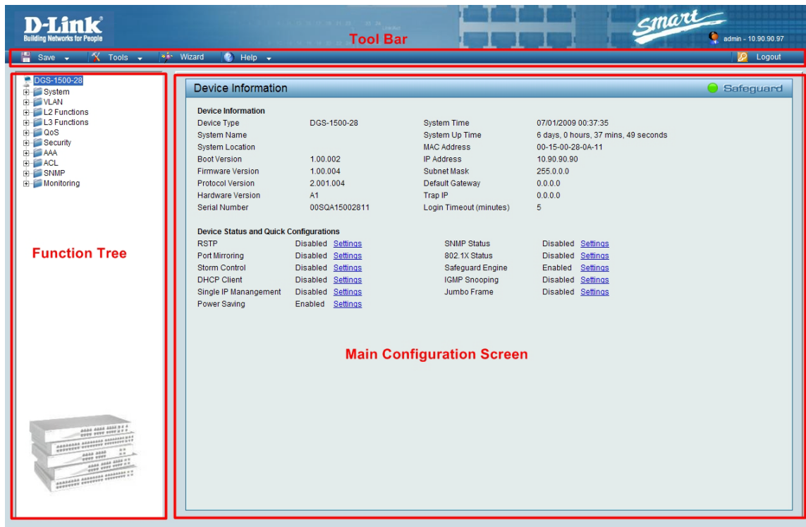
Figure 5.4 – Web-based Management
