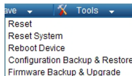
Figure 5.8 – Tool Menu
