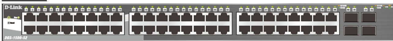
Figure 1.5 – DGS-1500-52 Front Panel
