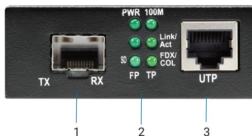
FIGURE 2-1. LHC210A FRONT PANEL
