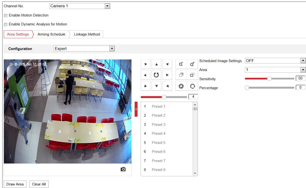
Figure 5-10 Motion Detection Settings-Expert
