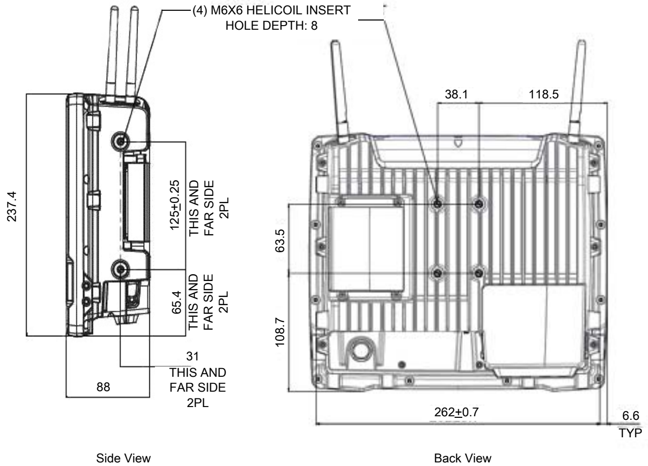
Figure 143 VC80x Drill Hole Dimensions
