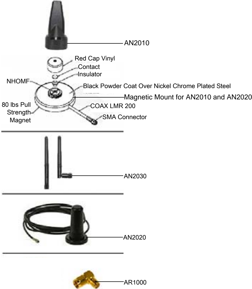
Figure 86 VC80x Antenna Options
