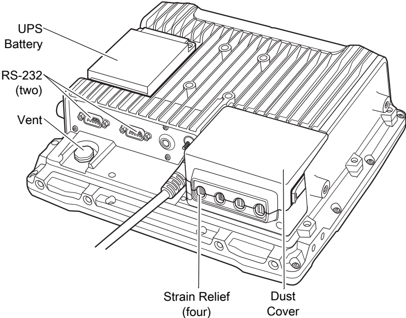
Figure 3 VC80x Back View with Dust Cover
