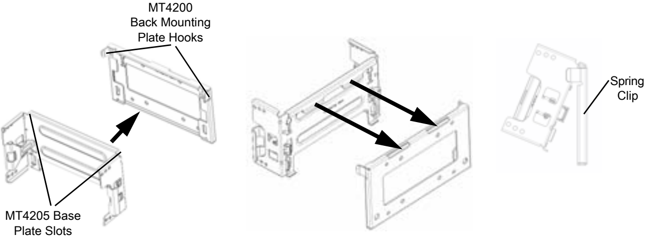
Figure 89 MT4200 Quick Release Mount Assembly
