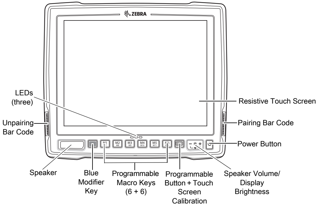
Figure 1 VC80x Front View
