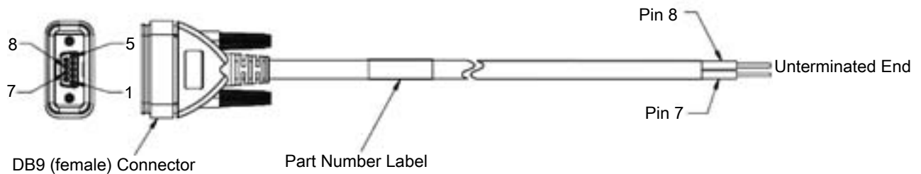
Figure 13 Screen Blanking DB9 Pin Configuration
