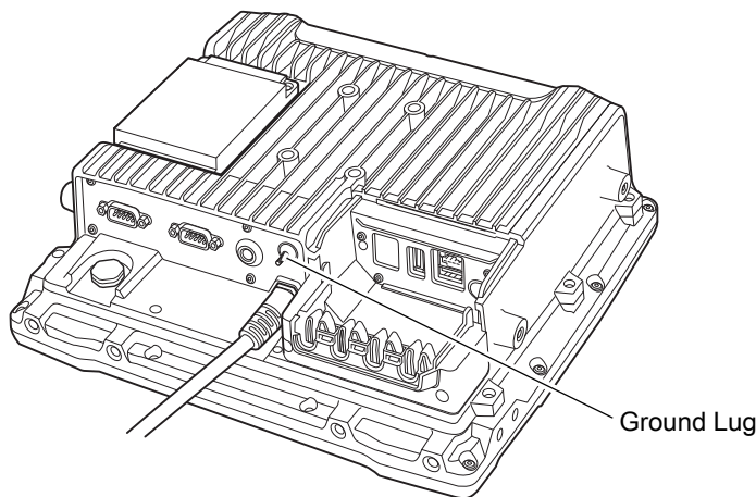
Figure 7 VC80x Ground Lug
