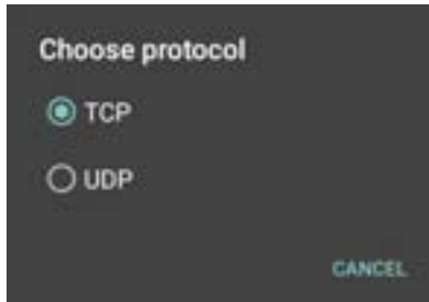
Figure 107 Protocol Selection
