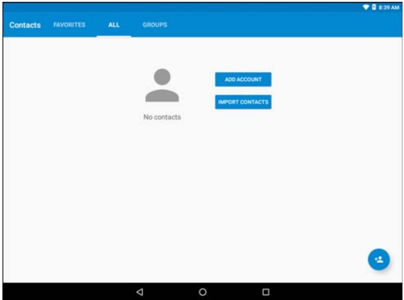
Figure 38 Contacts Screen
