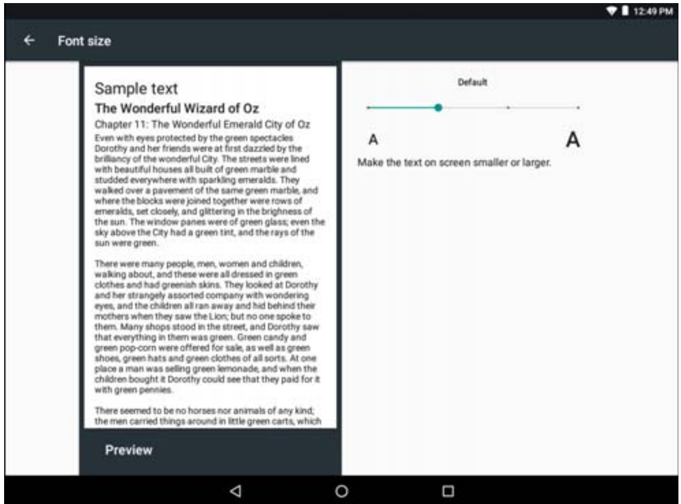
Figure 120 Font Settings
