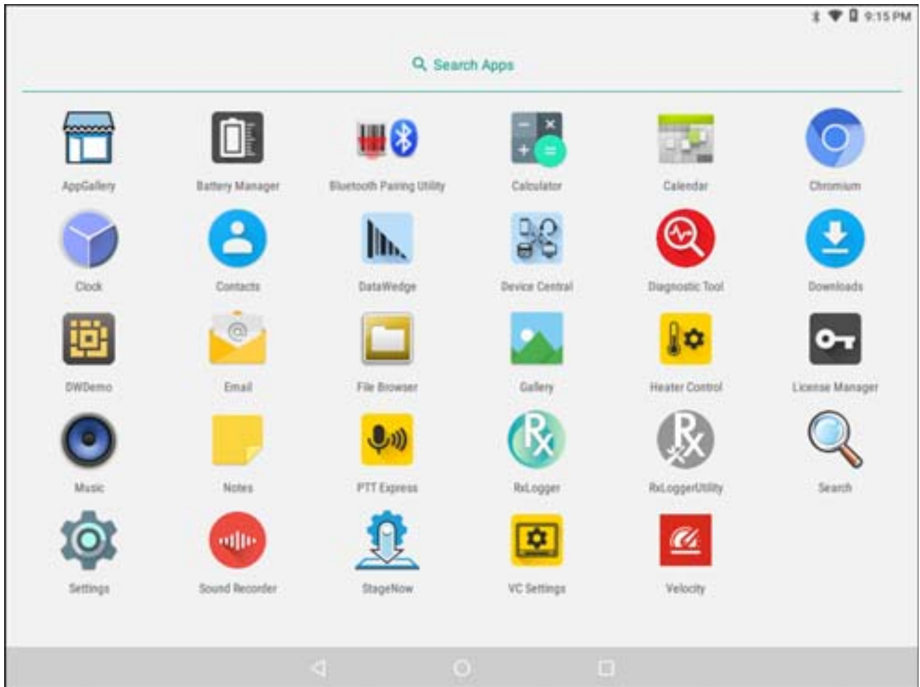
Figure 59 Velocity Icon
