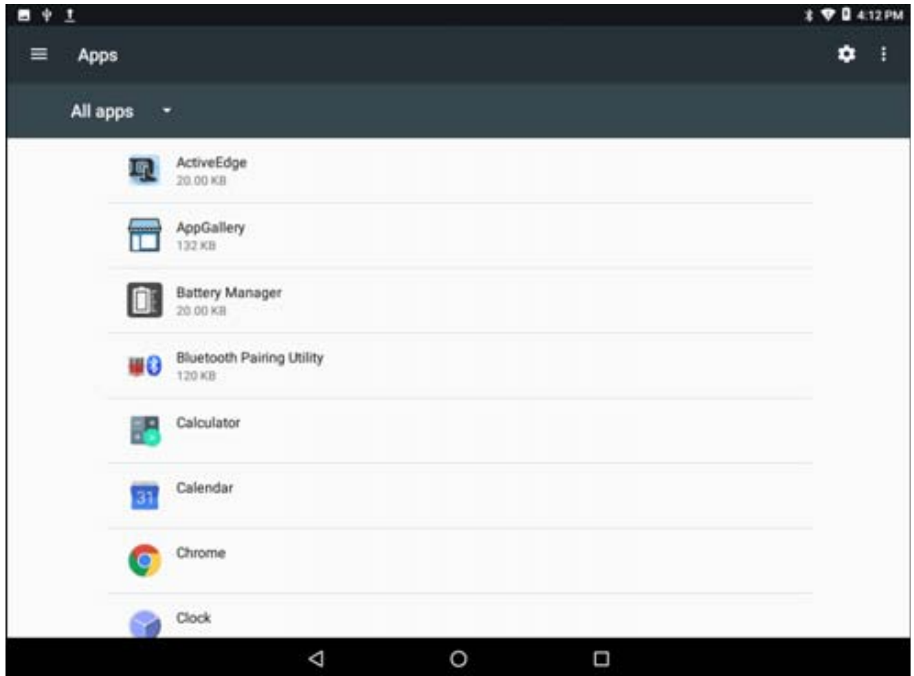
Figure 141 Apps Screen
