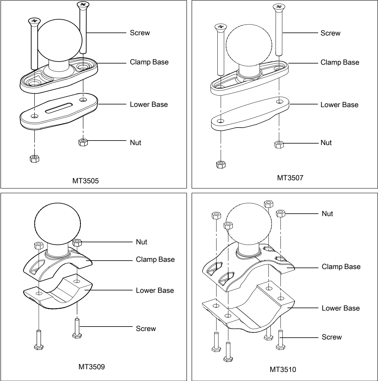
Figure 88 Optional Mount Kits
