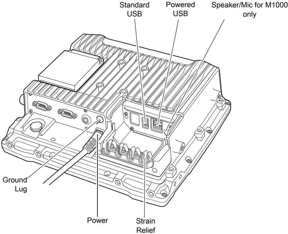
Figure 4 VC80x Back View without Dust Cover
