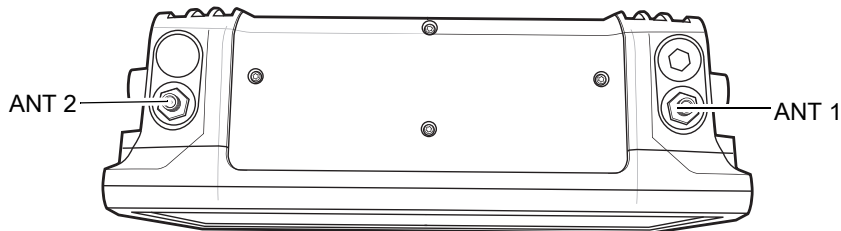
Figure 2 VC80x Top View
