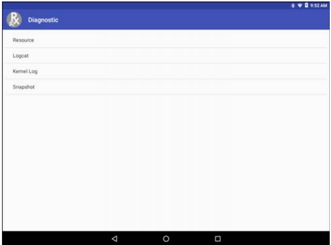
Figure 49 Diagnostic Window
