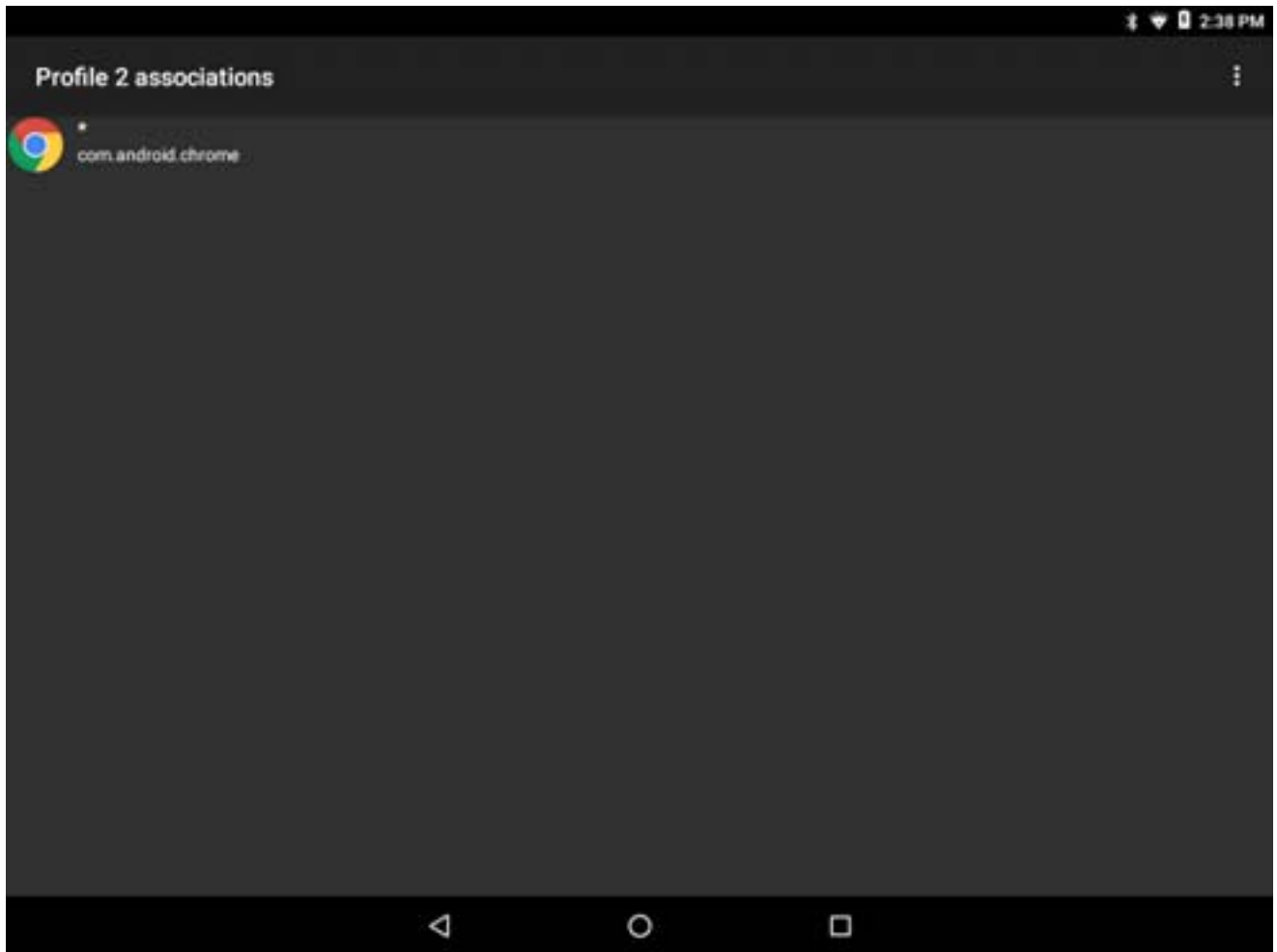
Figure 99 Selected Application/Activity
