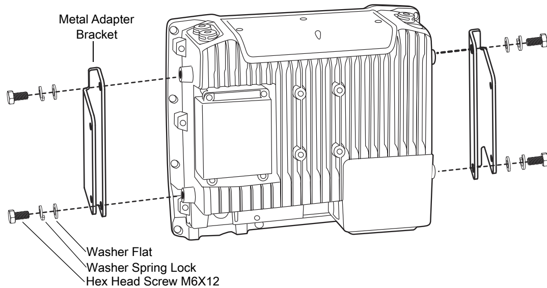
Figure 91 MT4210 Adapter Bracket Assembly
