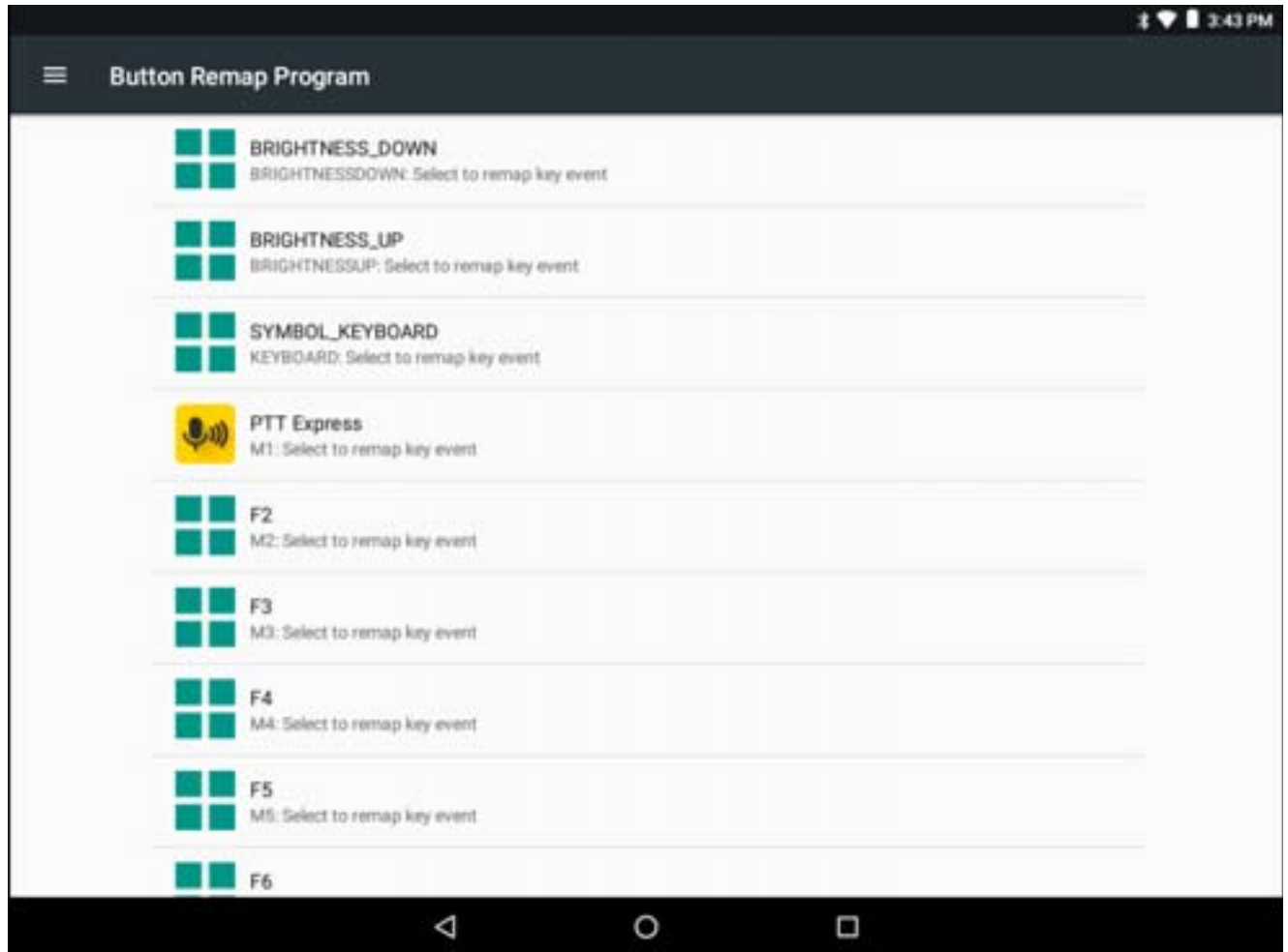
Figure 127 Remapped Button
