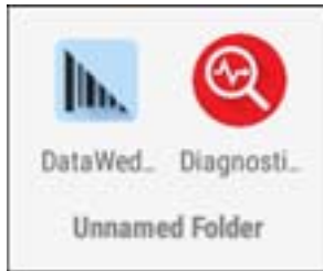
Figure 20 Open Folder
